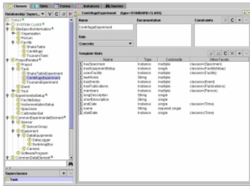
Figure 8. Preliminary version of NEES Data Model viewed using Protege2000
