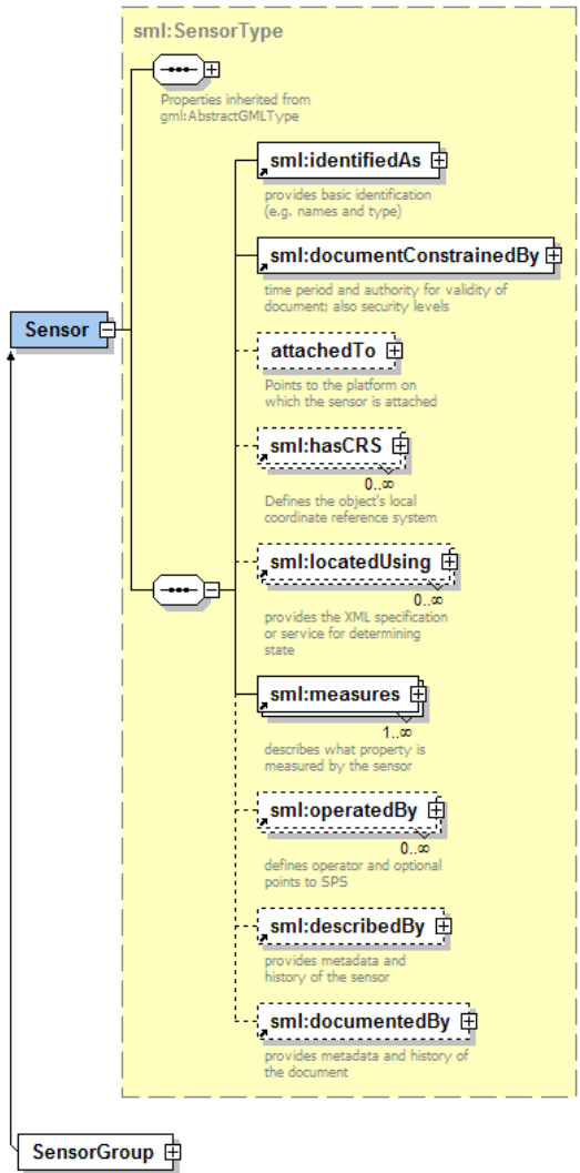
Figure 4. Schema diagram showing the highest level of the SensorML document structure [29].
